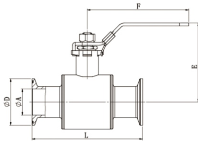
Quick-install Monobloc Straight-through Ball Valve (With Clamp) ●●●
